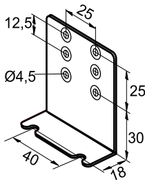
Mounting bracket angle Part No.: 803 799
