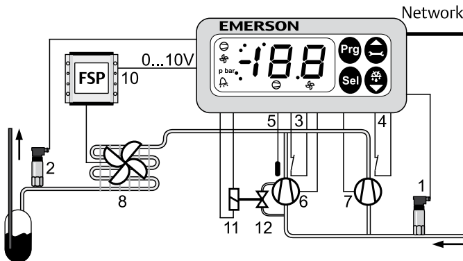
EC2-552 Condensing Unit Controller for 1 Digital Scroll and 1 single stage compressor
