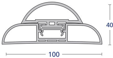
WP100+WPCS
