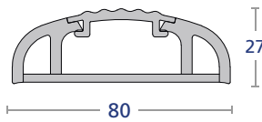
BUMPER 80 SUPERFLEX
